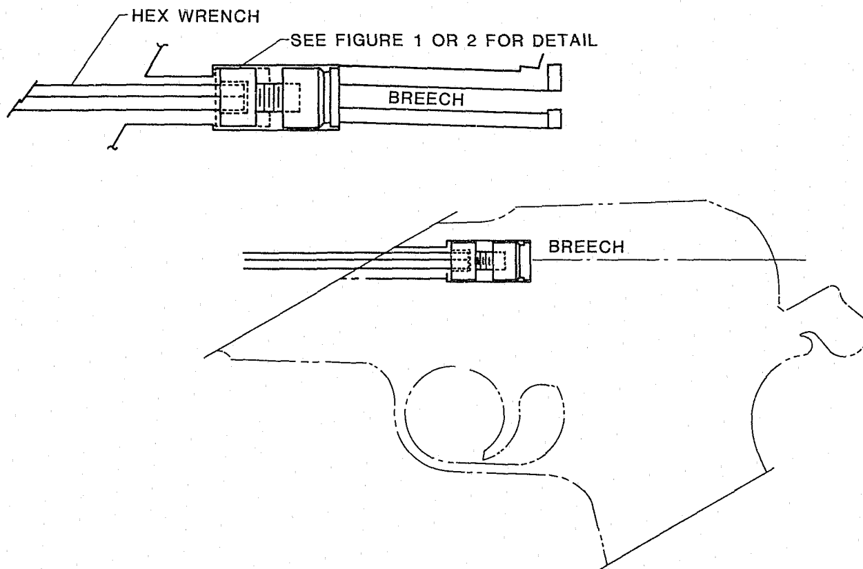
FIGURE 5. Headspace gage usage.
