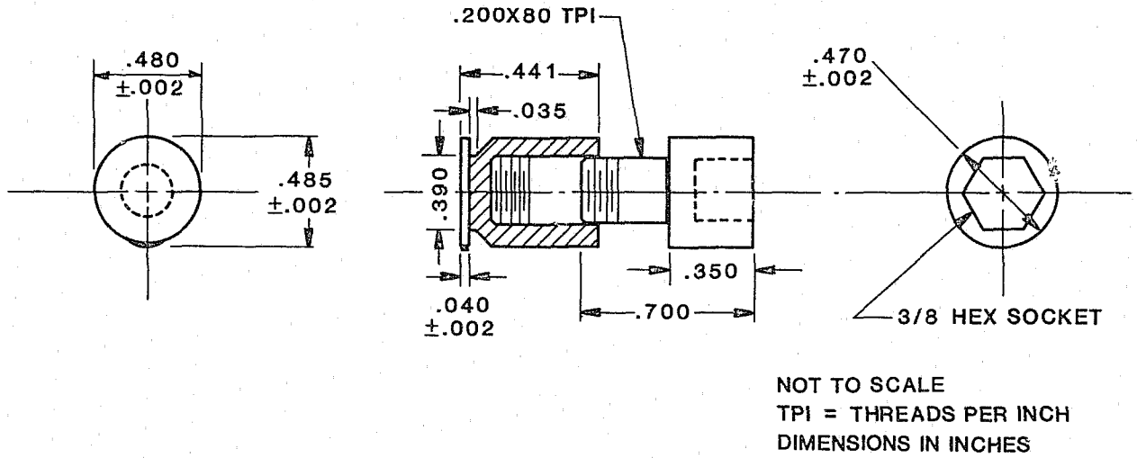
FIGURE 1. 9 mm Luger adjustable headspace gage.
