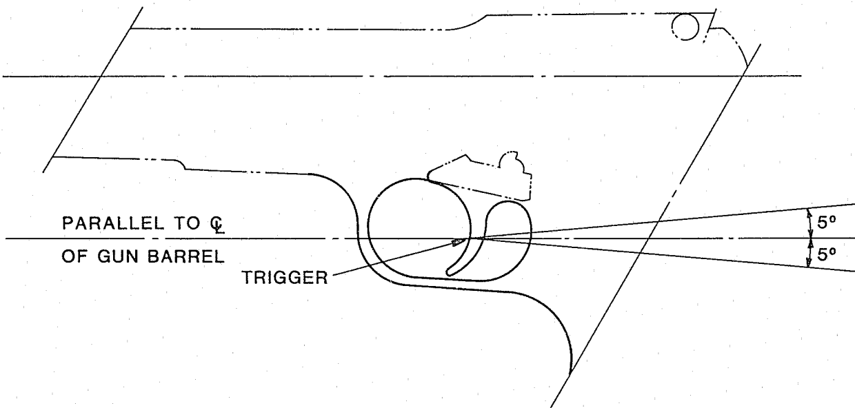
FIGURE 6. Trigger pull test.
