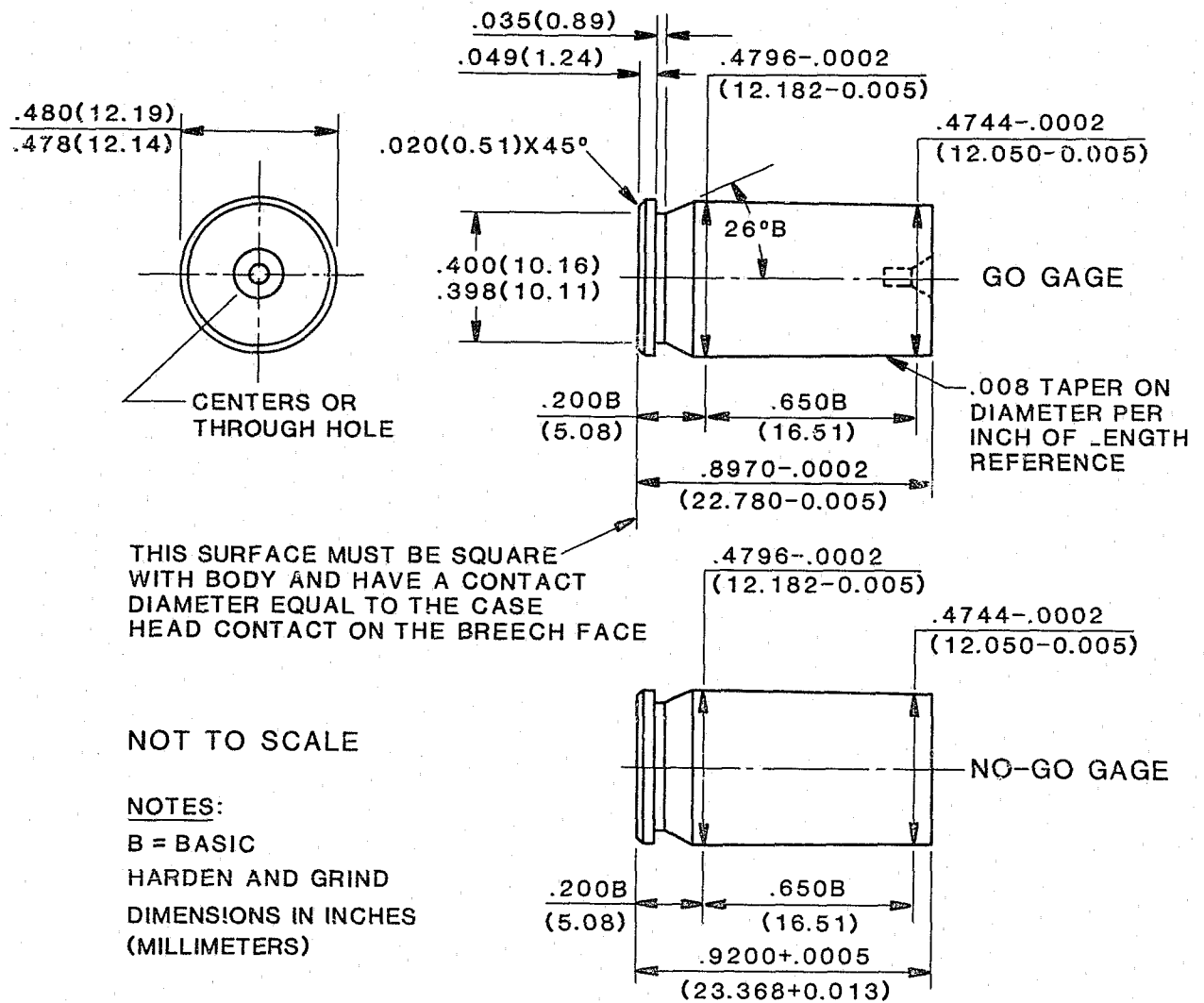
FIGURE 4. Go, no-go gages for 45 Automatic.
