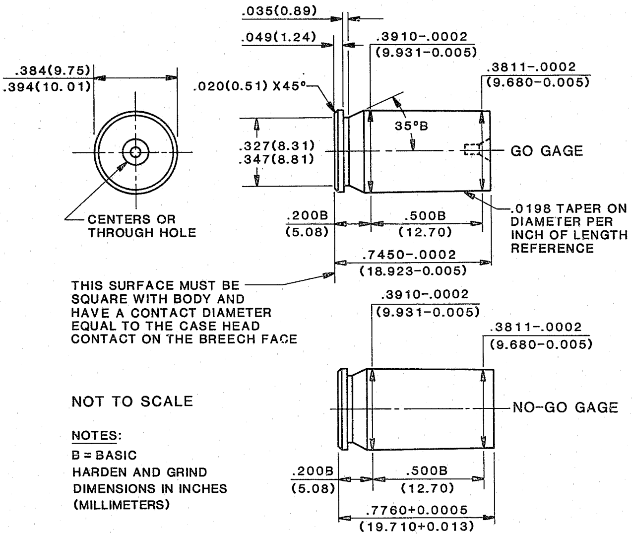
FIGURE 3. Go, no-go gages for 9 mm Luger.
