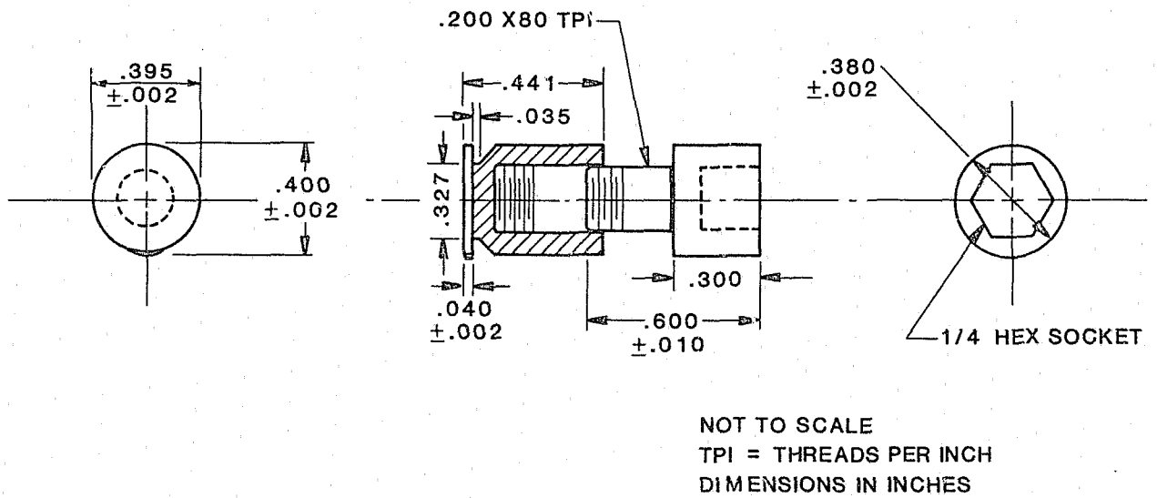
FIGURE 2. .45 Automatic adjustable headspace gage.
