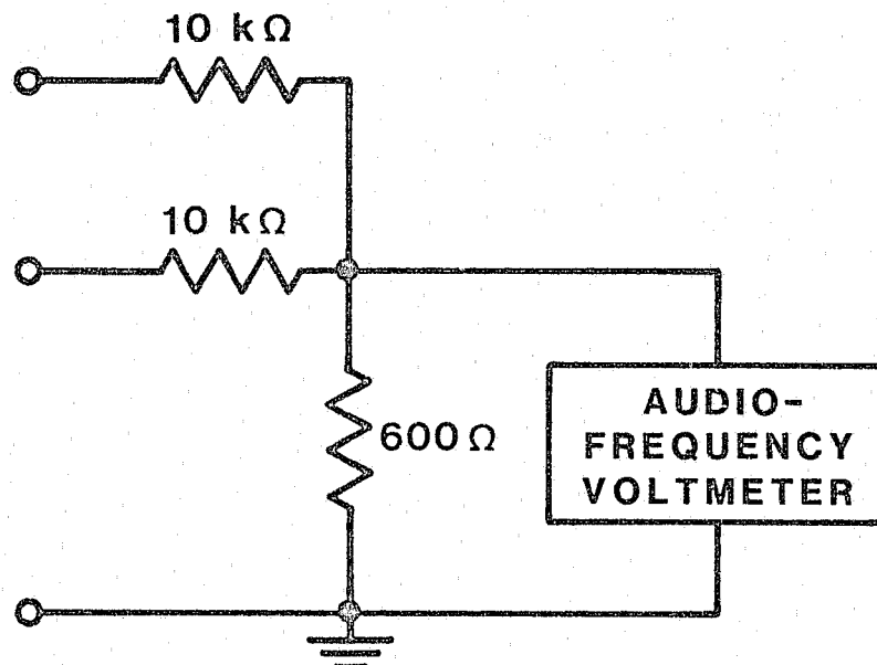
FIGURE 3. Block diagram for circuit used in the playback phase, record phase and track format measurements.
