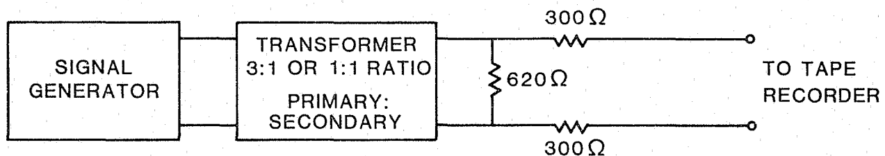
FIGURE 6. Block diagram for transformer circuit used in the high-level input impedance measurement.
