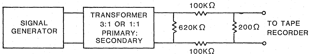
FIGURE 4. Block diagram for transformer circuit used in the microphone input, record-level indicator, overall frequency response, signal-to-noise ratio, interchannel crosstalk ratio, and recorded tape protection measurements.
