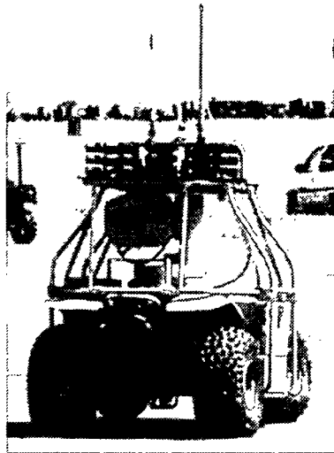
Figure 39. SARGE robot with Foster–Miller less-lethal weapon launcher.
