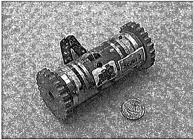
Figure 43. Scout robot.
