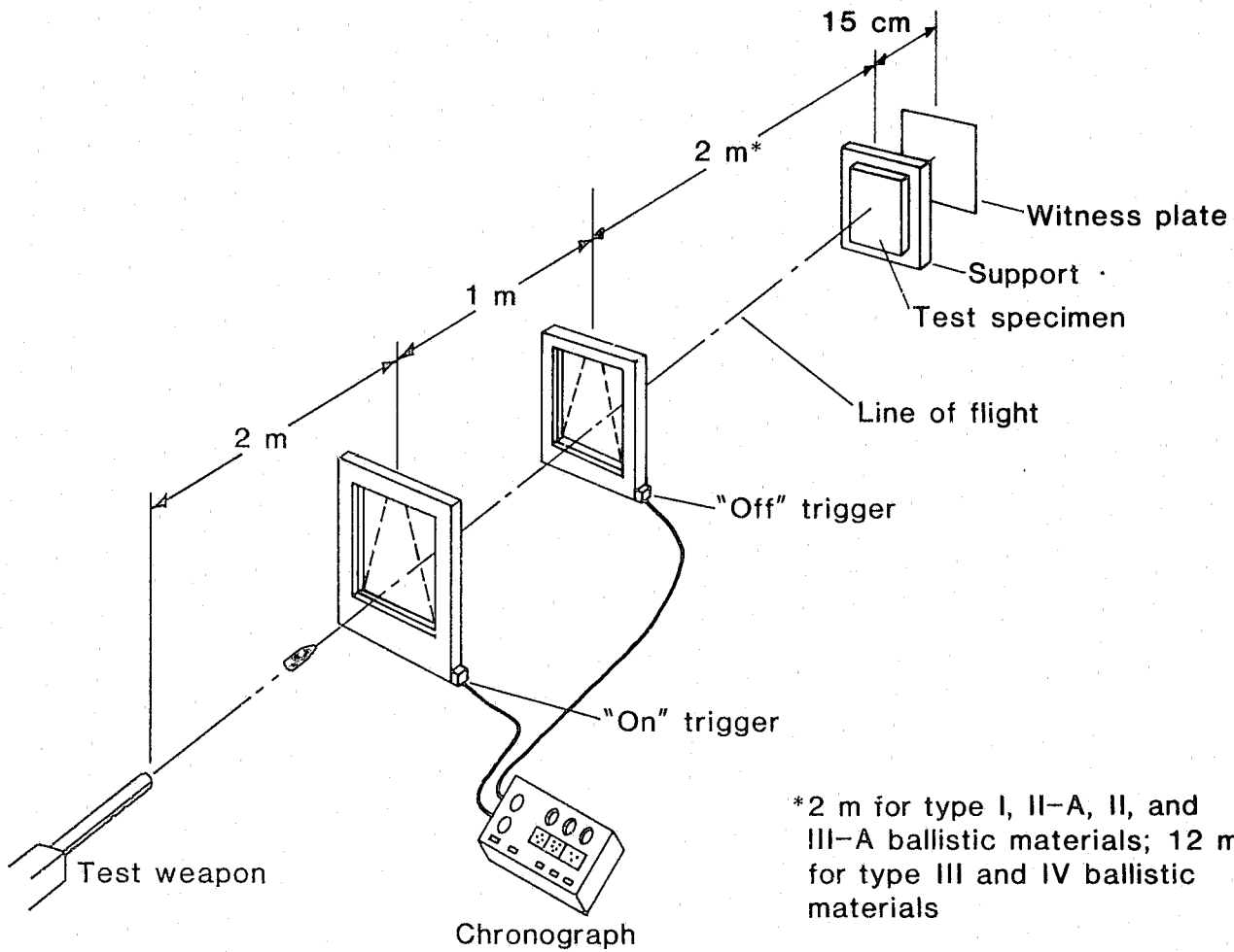
FIGURE 2. Ballistic test setup.
